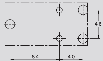
1 Form C
