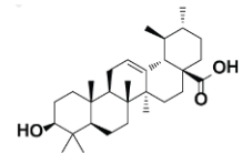
Ursolic acid
