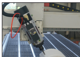
Italian HSD ATC 9KW Air Cool Spindle
